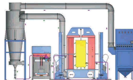
Fast color changing powder coating booth
