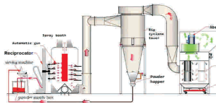
Powder spray booth system –Big cyclone serie
